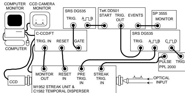
Fig. 2. Streak camera triggering configuration.
